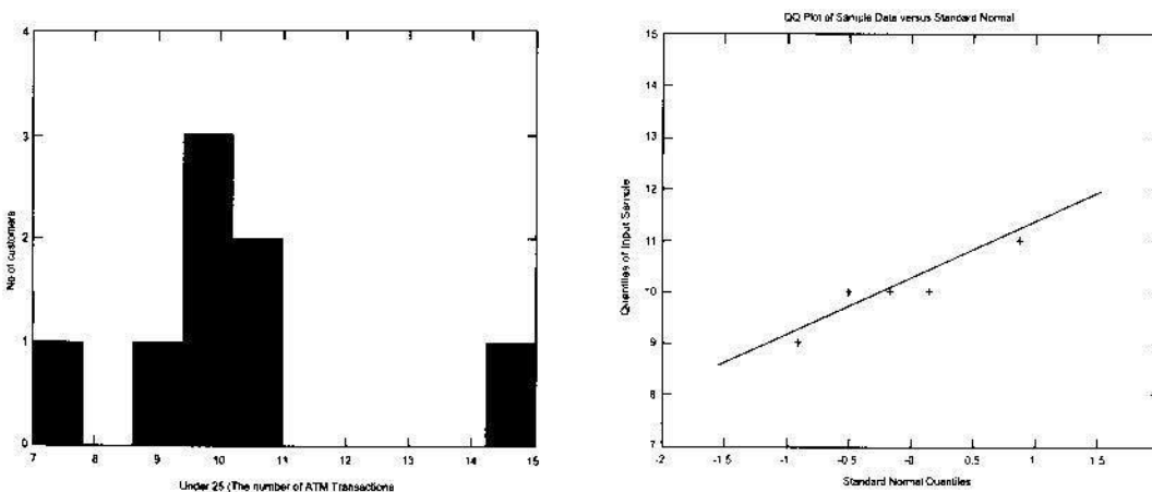
Figure III - Histogram and QQ plot of under 25
