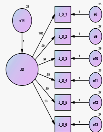
Fig. 4: Unidimensionality for JS
